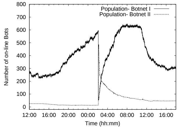
Figure 12: Migration of a botnet as observed by our IRC Tracker.
